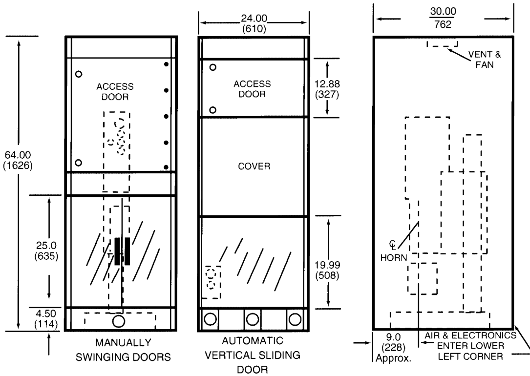
Standard Size 64" (1626 mm)H x 30" (610 mm)W x 30" (762 mm)D
