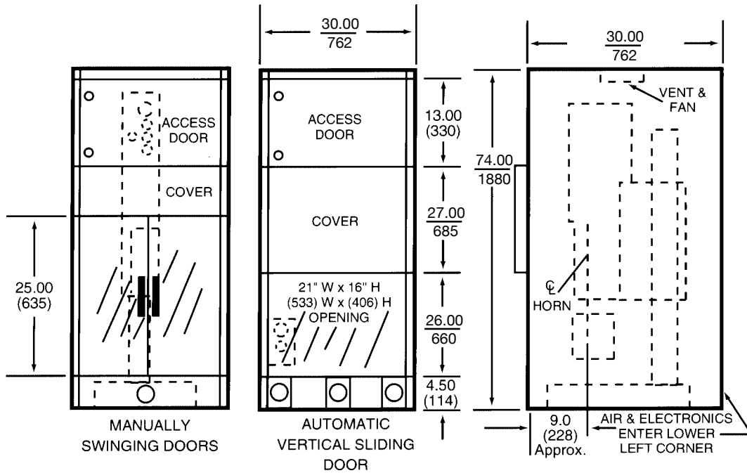
Standard Size 74" (1880 mm)H x 30" (762 mm)W x 30" (762 mm)D
